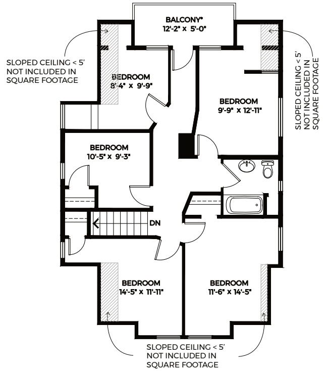
TOP FLOOR CEILING HEIGHT: 7'-10"
